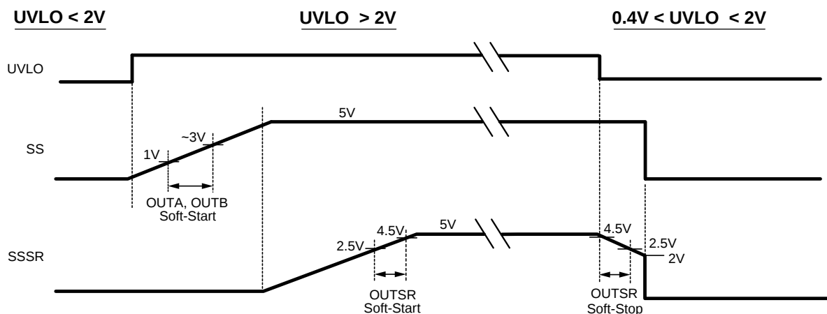
Figure 21. Soft-Start/Soft-Stop Timing
