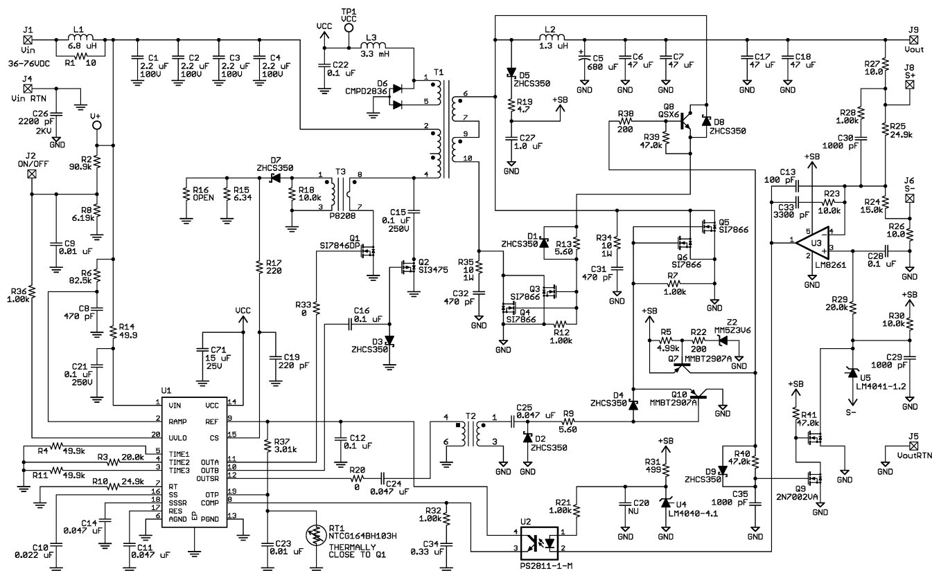
Figure 34. Application Circuit
